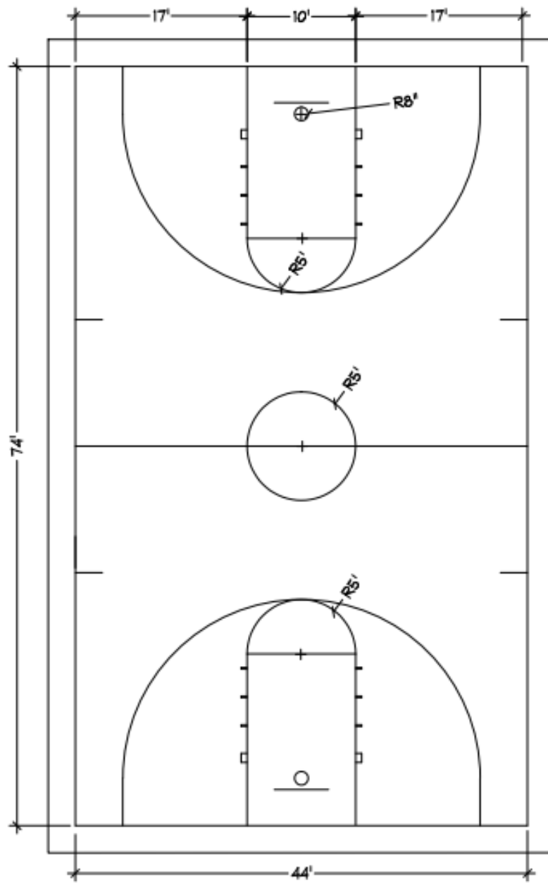
PLAN VIEW
