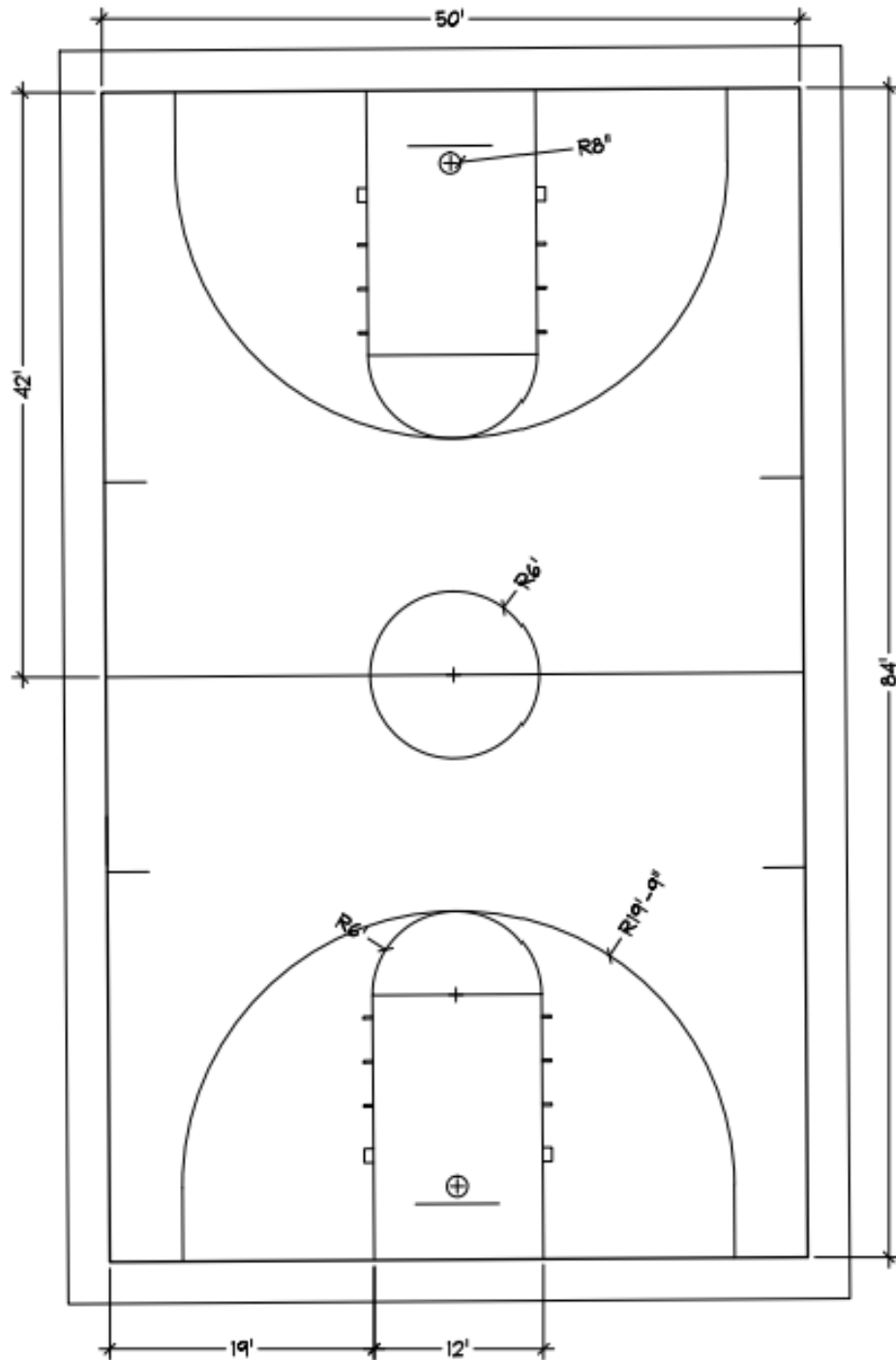
PLAN VIEW
