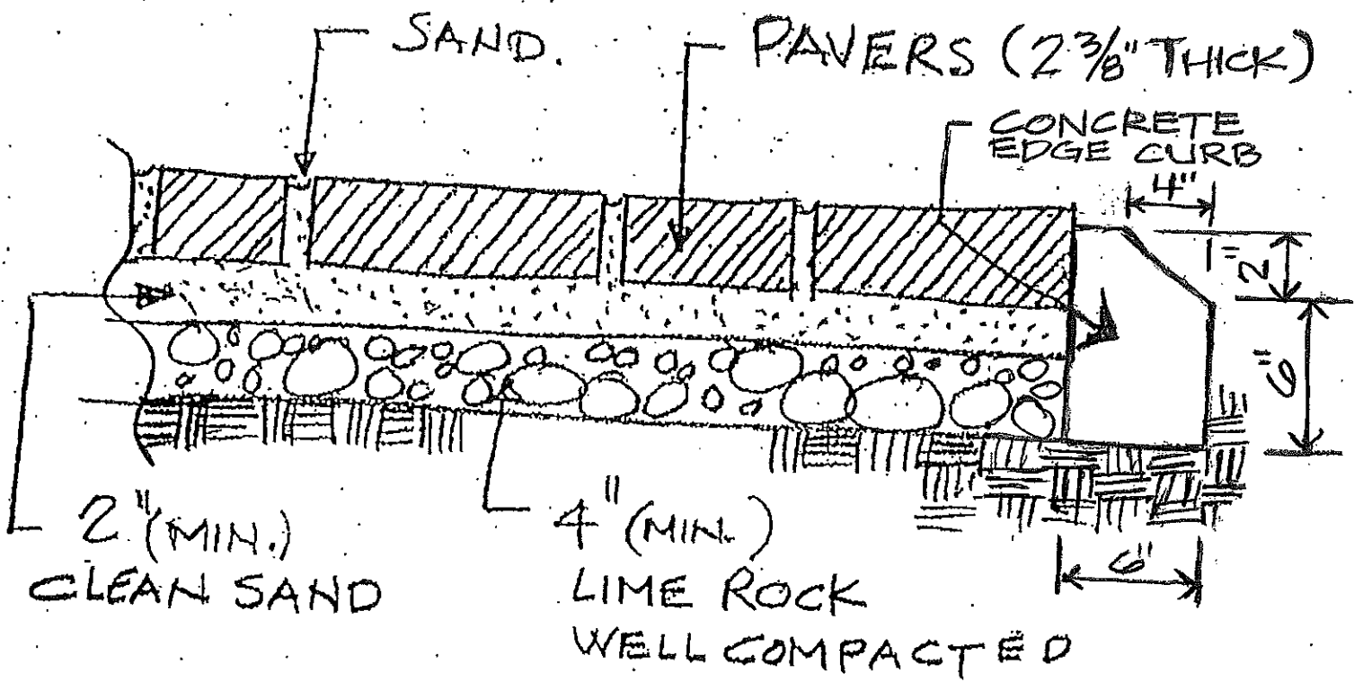
SECTION - DETAIL N.T.S (PAVERS INSTALLATION)
