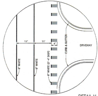
DETAIL H ADJACENT TO DRIVEWAY NTS
