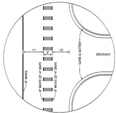
DETAIL I ADJACENT TO DROP-OFF LANE NTS
