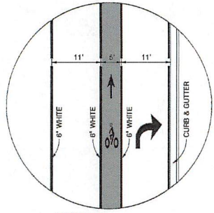
DETAIL G ADJACENT TO RIGHT TURN LANE NTS
