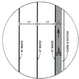
DETAIL F ADJACENT TO CURB & GUTTER NTS
